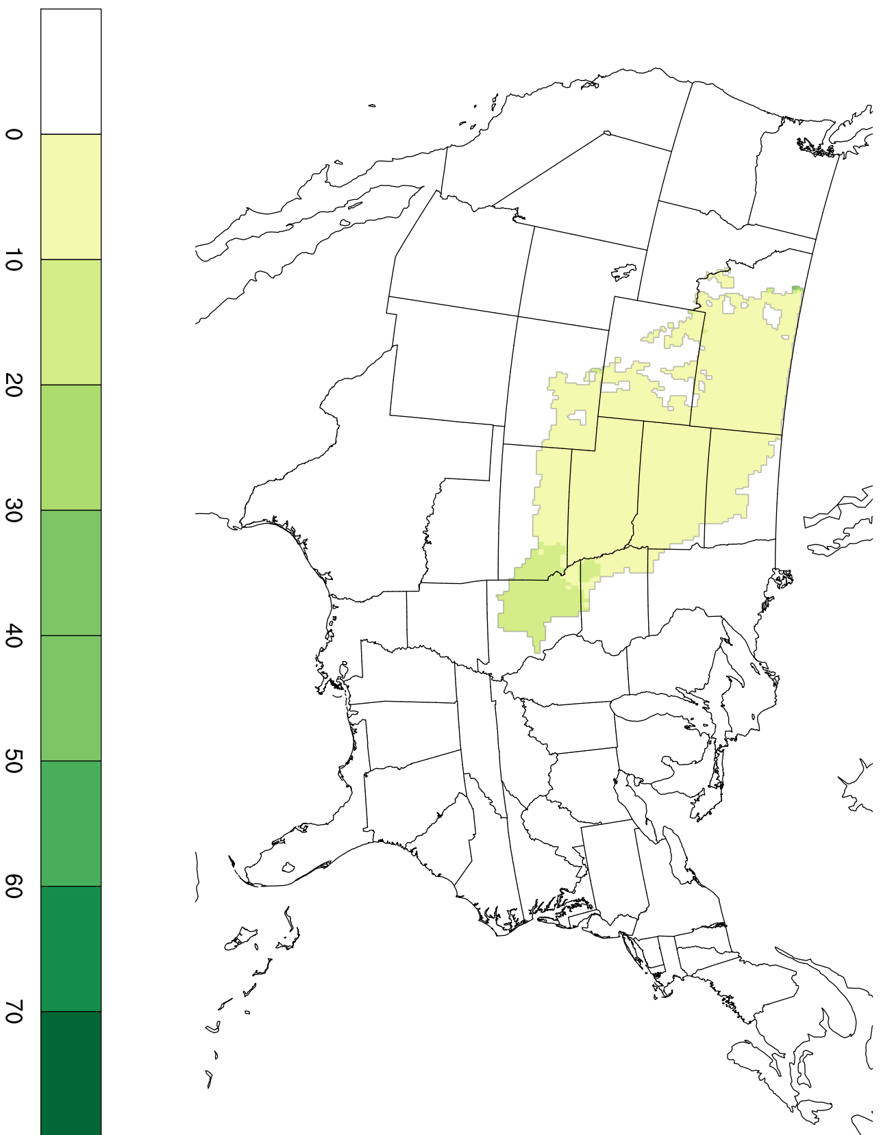
prism_base_25km_t150_morb
