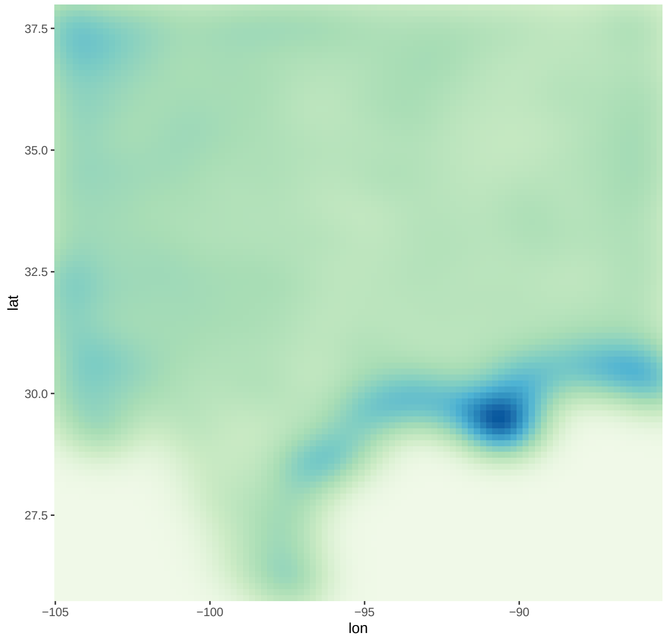
Object Scatterplot
