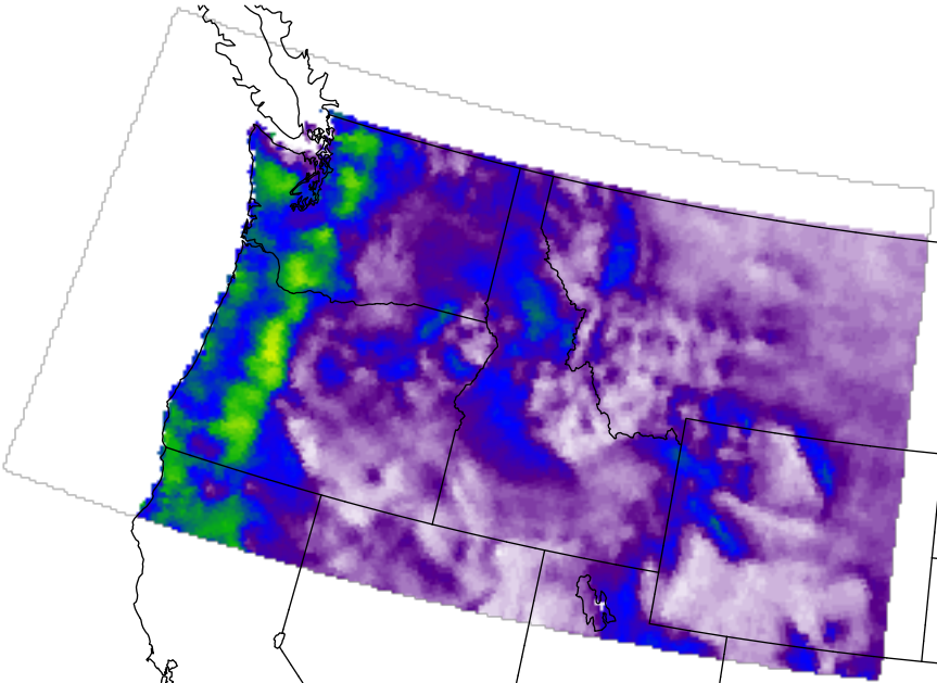
regcm4_gfdl_base_12km_1981_2005_t25
