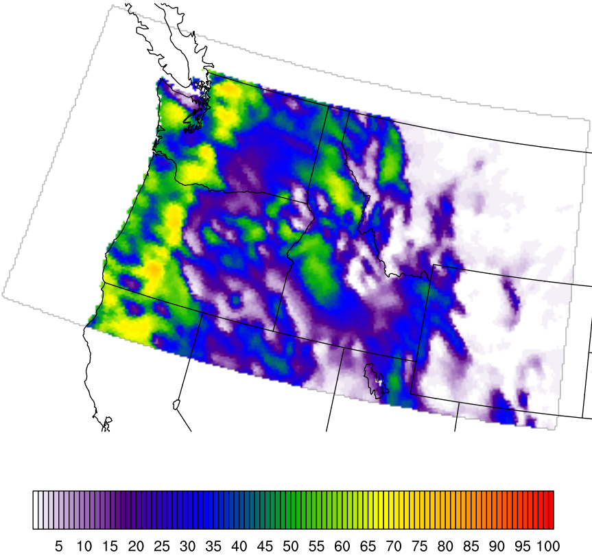
regcm4_gfdl_base_12km_1981_2005_t25
