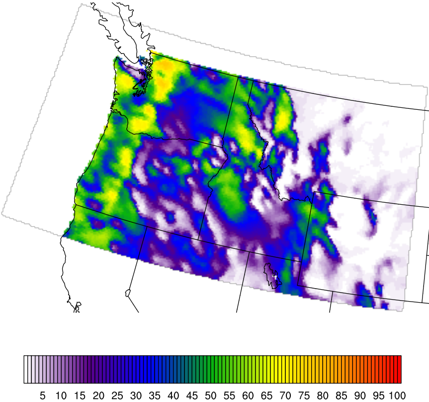
regcm4_erai_base_12km_1991_2010_t25
