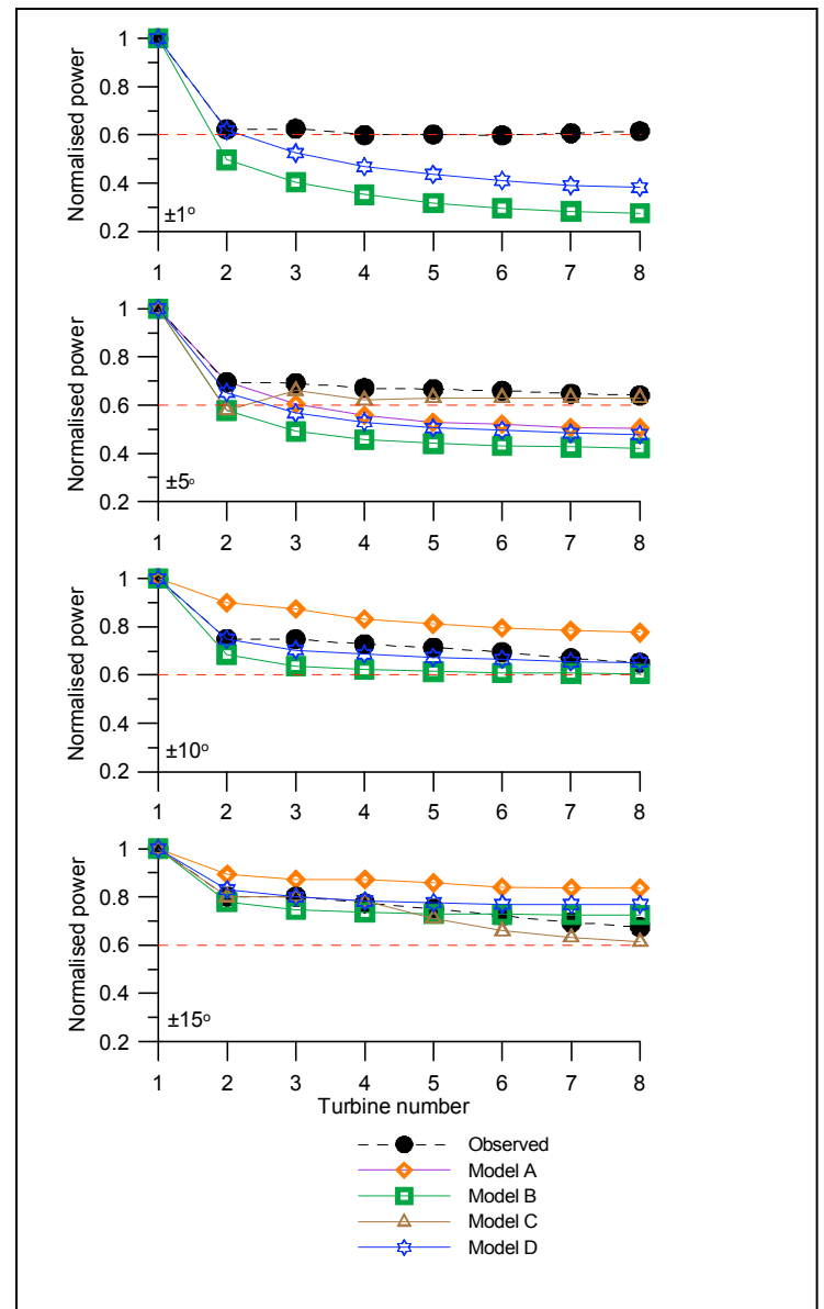
Figure 8. Adapted from (Barthelmie et al. 2008). The observations are from the Horns Rev wind plant taking data from direction 274^\circ (exactly down a row of wind turbines) with different sector widths. The model results shown are from the UPWIND project incorporating both wind plant (parameterized) and CFD models.
