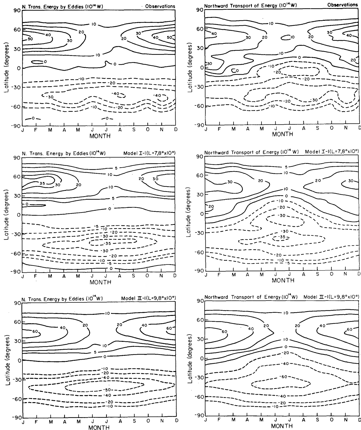
FIG. 38. Northward transport of energy by eddies (left) and by eddies plus mean circulation (right). Observations are from Oort (1982).
