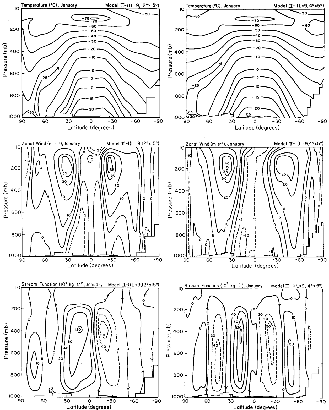
FIG. 41. Zonal-mean temperature, zonal wind and streamfunction for 12^\circ \times 15^\circ (left) and 4^\circ \times 5^\circ (right) horizontal resolution of Model II. Model results for 8^\circ \times 10^\circ resolution and observations are given in Figs. 20, 29 and 31.
