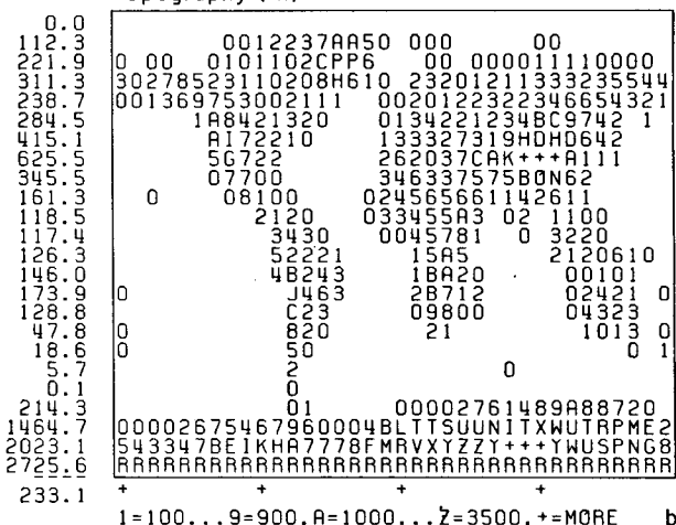
FIG. 4. Digital maps of land coverage and topography for 8^\circ \times 10^\circ model. A blank on either map is identically zero. For land coverage 0 is 0–5%, 1 is 5–15%, A is 95–100% and X is exactly 100%. For topography 0 is 0–50 m, 1 is 50–150 m and + is more than 3550 m. Longitudinal averages are on the left, above the area-weighted global average.
