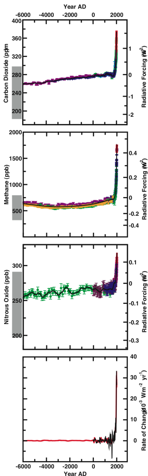
FIGURE SPM-1. Atmospheric concentrations of carbon dioxide (CO 2 ), methane (CH 4 ), nitrous oxide (N 2 O), and the rate of change in their combined radiative forcing. In the upper three panels, symbols denote measurements from ice cores or atmospheric samples and smoothed values are denoted by a solid line. Grey bars show the ranges associated with changes from ice ages to intervening warm periods over the past 650,000 years. Estimated radiative forcings due to changes since 1750 are indicated on the right hand side. The rate of change in total radiative forcing from all three gases is shown in the bottom panel with different amounts of smoothing corresponding to the averaging occurring in low accumulation (red) and high accumulation (black) ice cores. [Figure 6.4]
