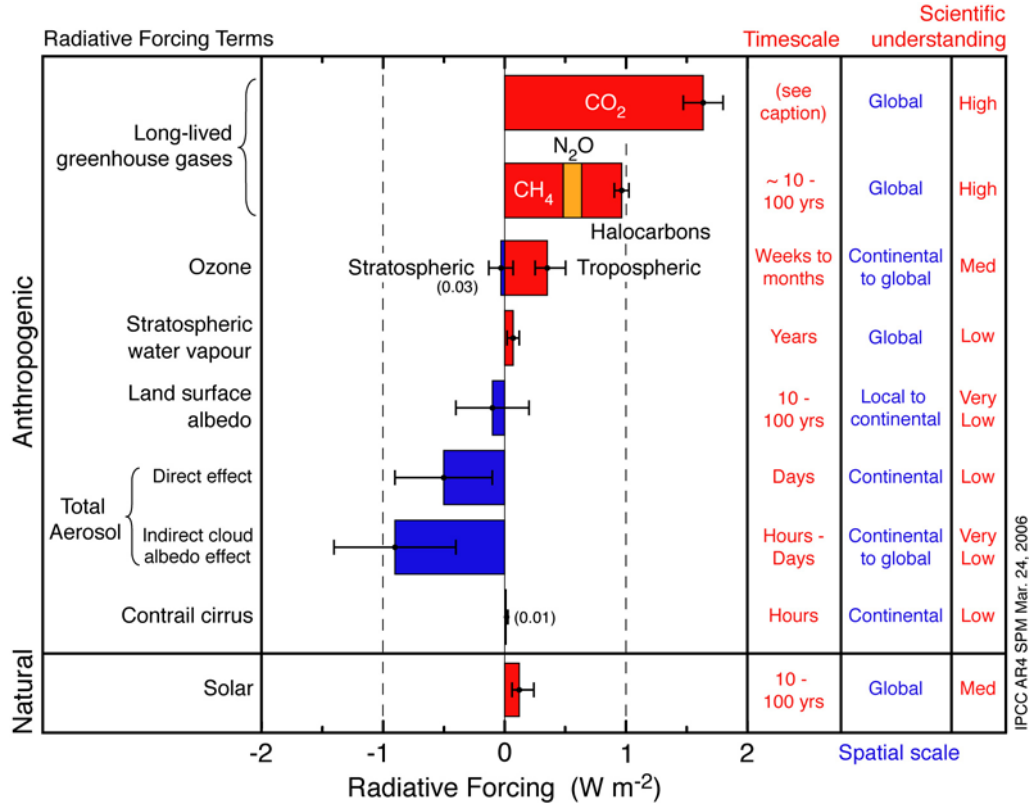
FIGURE SPM-2. Global-mean radiative forcings and their 65% (1 sigma) uncertainty range for various agents and mechanisms. Columns on the right hand side specify: (Timescale) the approximate duration of variation/change in the agent; (Spatial scale) typical geographical extent of the forcing; (Scientific understanding) scientific confidence level as explained in section 2.9. No CO 2 timescale is given as its removal from the atmosphere involves many processes and cannot be expressed accurately with a single lifetime. Errors for CH 4 , N 2 O, and halocarbons have been combined. [Figure 2.24]
