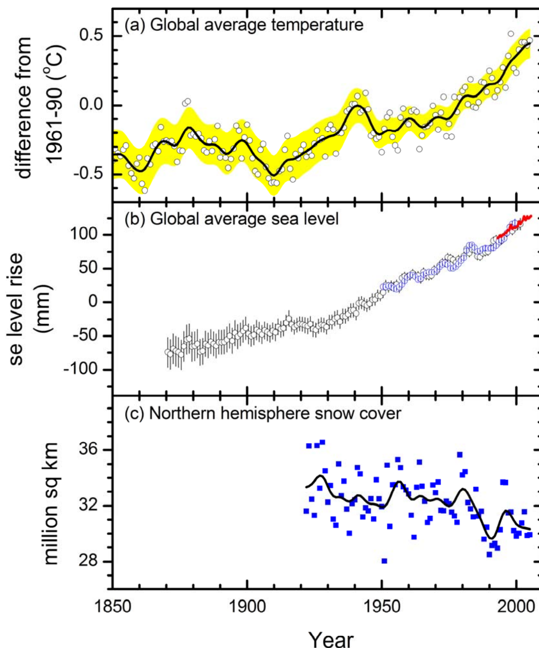
FIGURE SPM-3. Changes in global mean temperature, sea level, and snow cover area. Panel (a) shows global mean temperatures as annual values (open circles) and a smoothed curve (black line) with uncertainty in the smoothed curve shown as a yellow shaded area. The temperature change from the first 70 years of the instrumental record (1850–1919) to the last 5 years (2001–2005) is 0.78 \pm 0.18^\circ\text{C} . Panel (b) shows global mean sea level rise from 1870 to 2001 from tide gauge data (black and blue circles) and recent satellite measurements (red line) as discussed in Section 5.5. Panel (c) shows estimates of April
