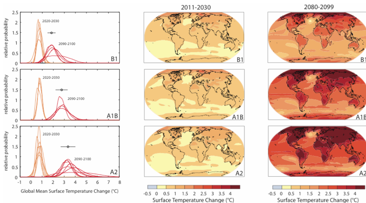
FIGURE SPM-5. Projected temperature changes for the early and late 21st century relative to the period 1980–1999. The central and right panels show the multi-model mean projections for the B1 (top), A1B (middle) and A2 (bottom) SRES scenarios averaged over 20-year periods 2011–2030 (central) and 2080–2099 (right). The left panel shows corresponding uncertainties as the relative probabilities in estimated global mean warming from several different studies for periods 2020–2030 and 2090–2100. [Figures 10.3.5 and 10.5.7.]
