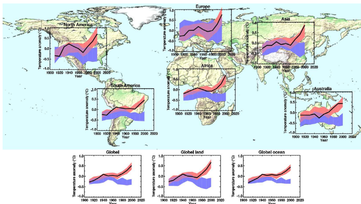
FIGURE SPM-4. Continental- and global-scale decadal surface air temperature anomalies for 1906–2005, relative to the 1901–1997 period, compared to model simulations. Black lines indicate observed changes. Blue bands show the 5–95% range for 19 simulations using only natural forcings and red bands show that range for 51 model simulations using both natural and anthropogenic forcings. [Question 9.2, Figure 1]
